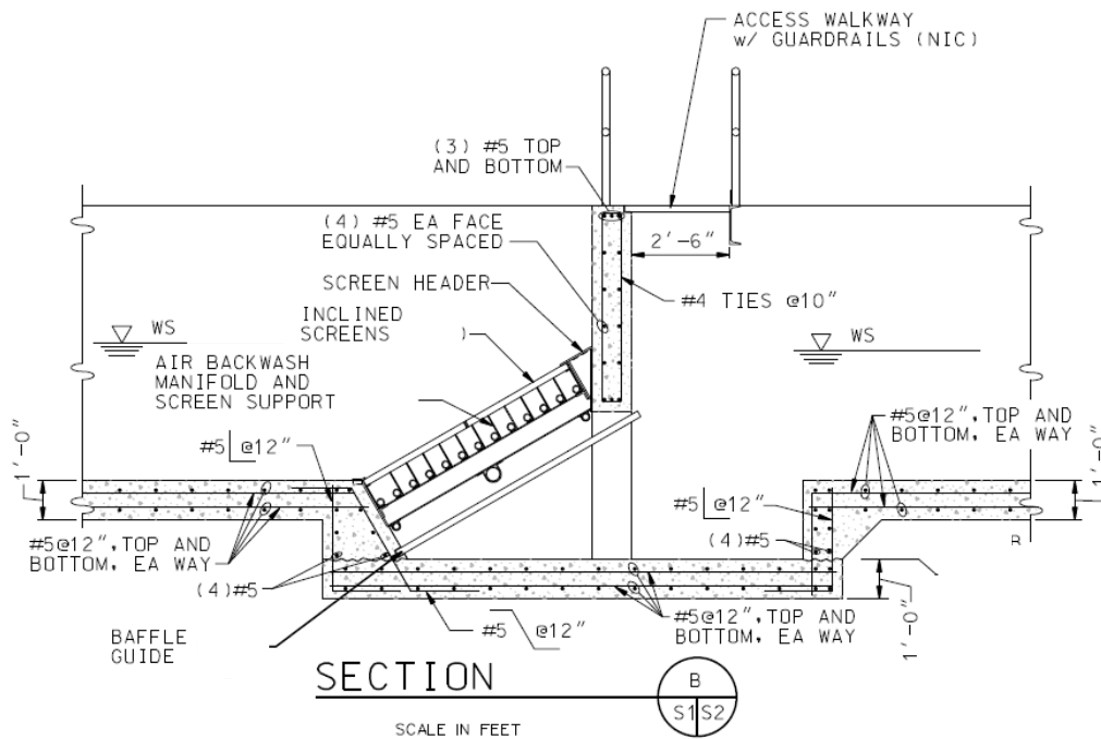
Figure 4-10 Typical Inclined Flat-Plate Screen
